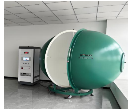
Integrating Sphere
